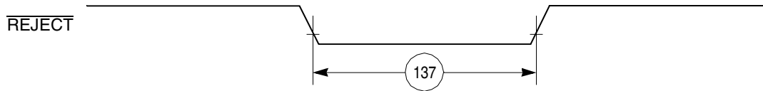
Figure 65. CAM Interface \overline{\text{REJECT}} Timing Diagram
